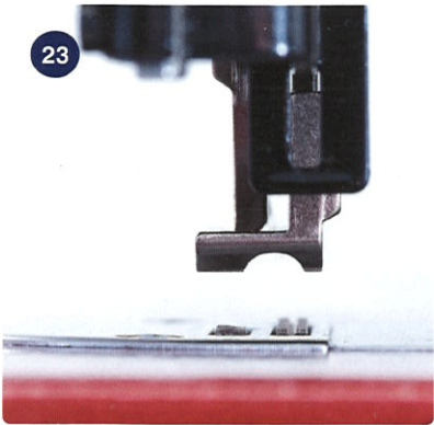
> LS-1 welting tunnel in presser foot (back view)
