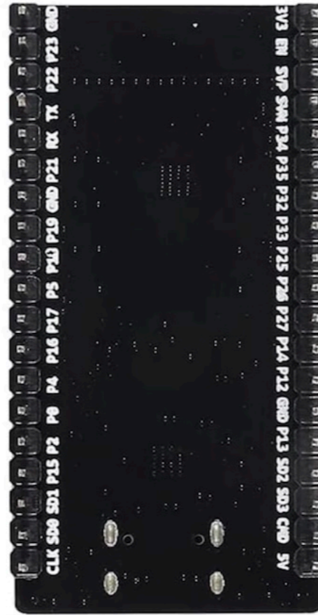
ESP32 38 pin
